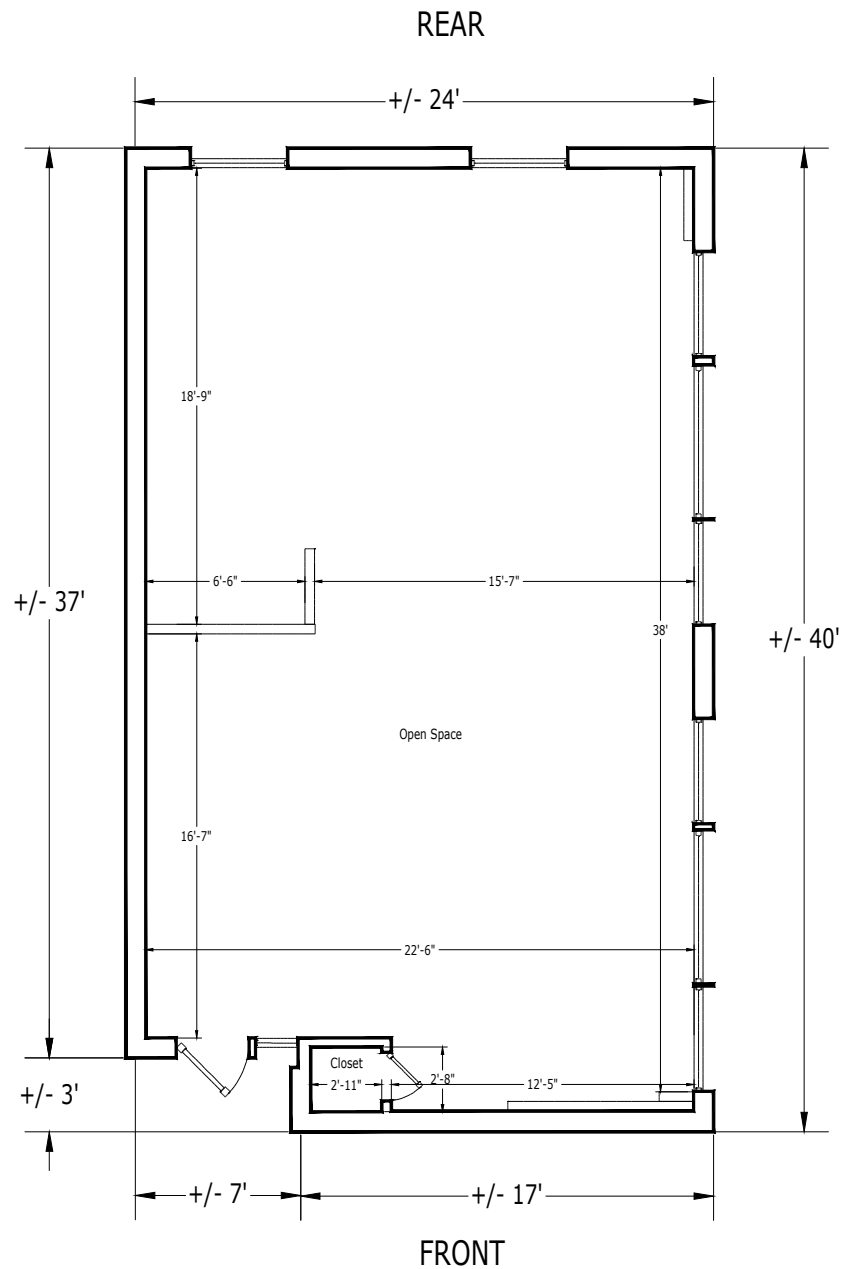
1 GROUND FLOOR
